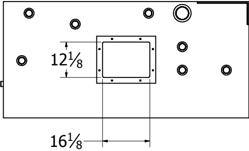
Inner Tank Showing Cut Out Detail
