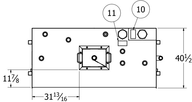
Inner Tank Showing Cut Out Detail
